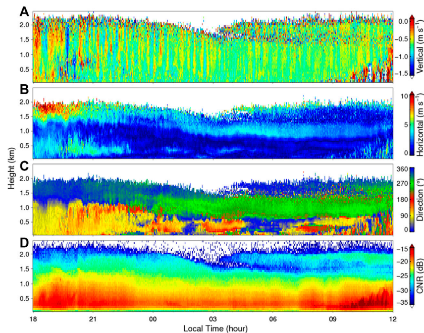
FIGURE 9 | A case of gravity wave process detected by C-DWL. (A) Vertical wind, (B) horizontal wind speed, (C) horizontal wind direction, and (D) CNR in vertical obtained by the CDL.
